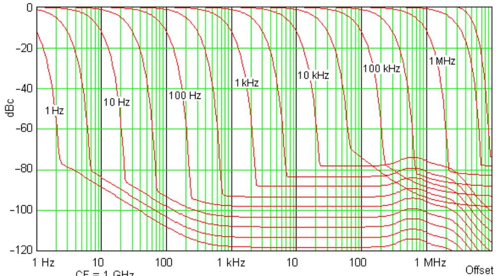
Nominal Dynamic Range vs. Offset Frequency vs. RBW(SN prefix \geq MY/SG/US5233, ship standard with N9020A-EP2) [Plot]
