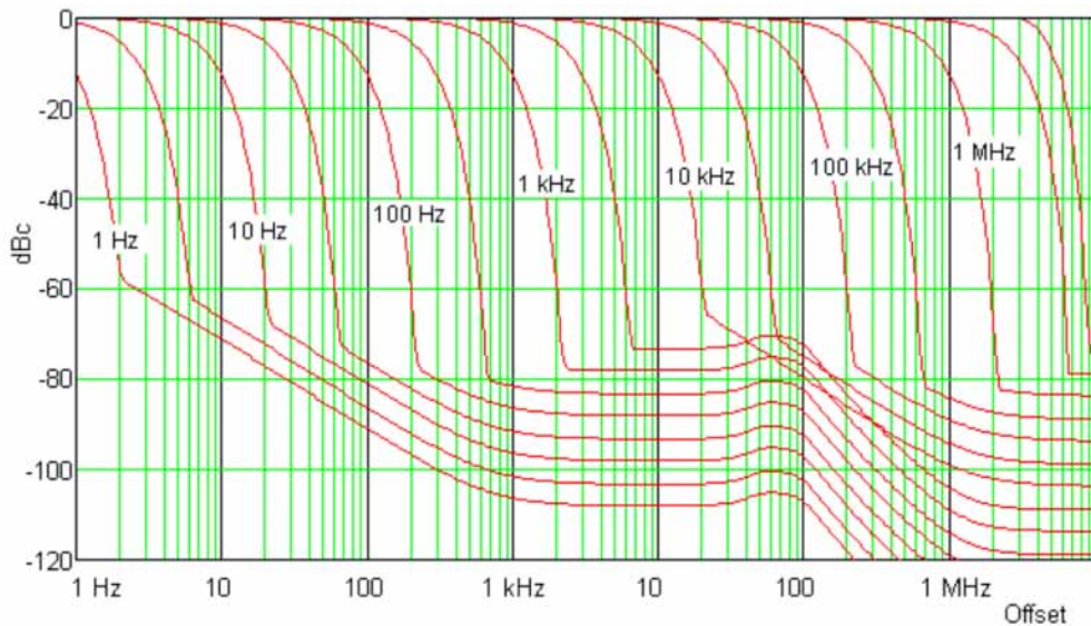
Nominal Dynamic Range vs. Offset Frequency vs. RBW (SN prefix < MY/SG/US5233) [Plot]
