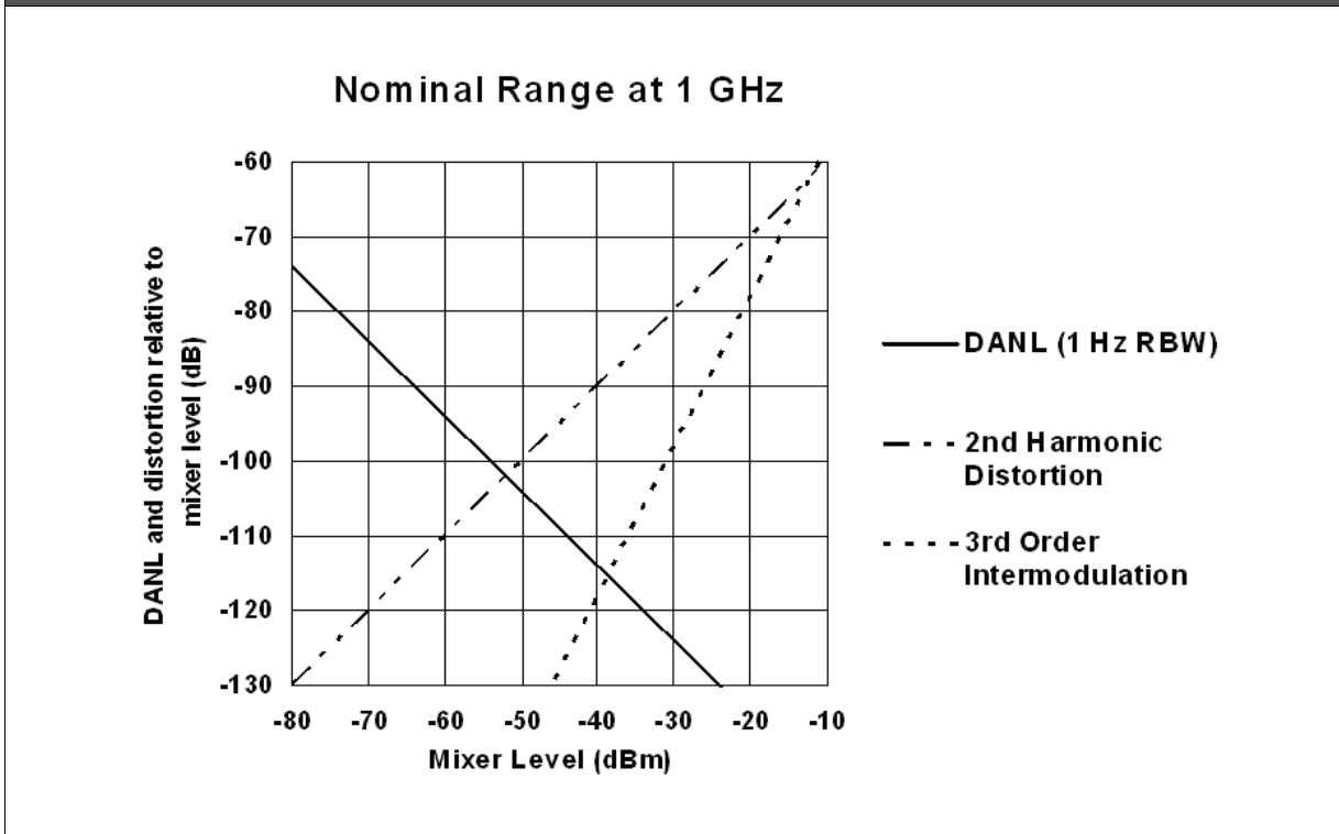
Nominal Dynamic Range at 1 GHz [Plot]
