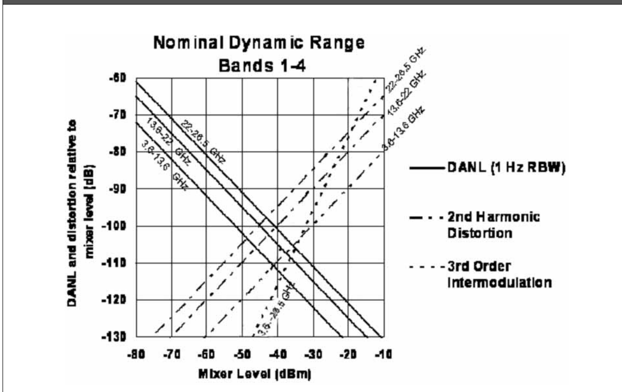
Nominal Dynamic Range Bands 1-4 [Plot]
