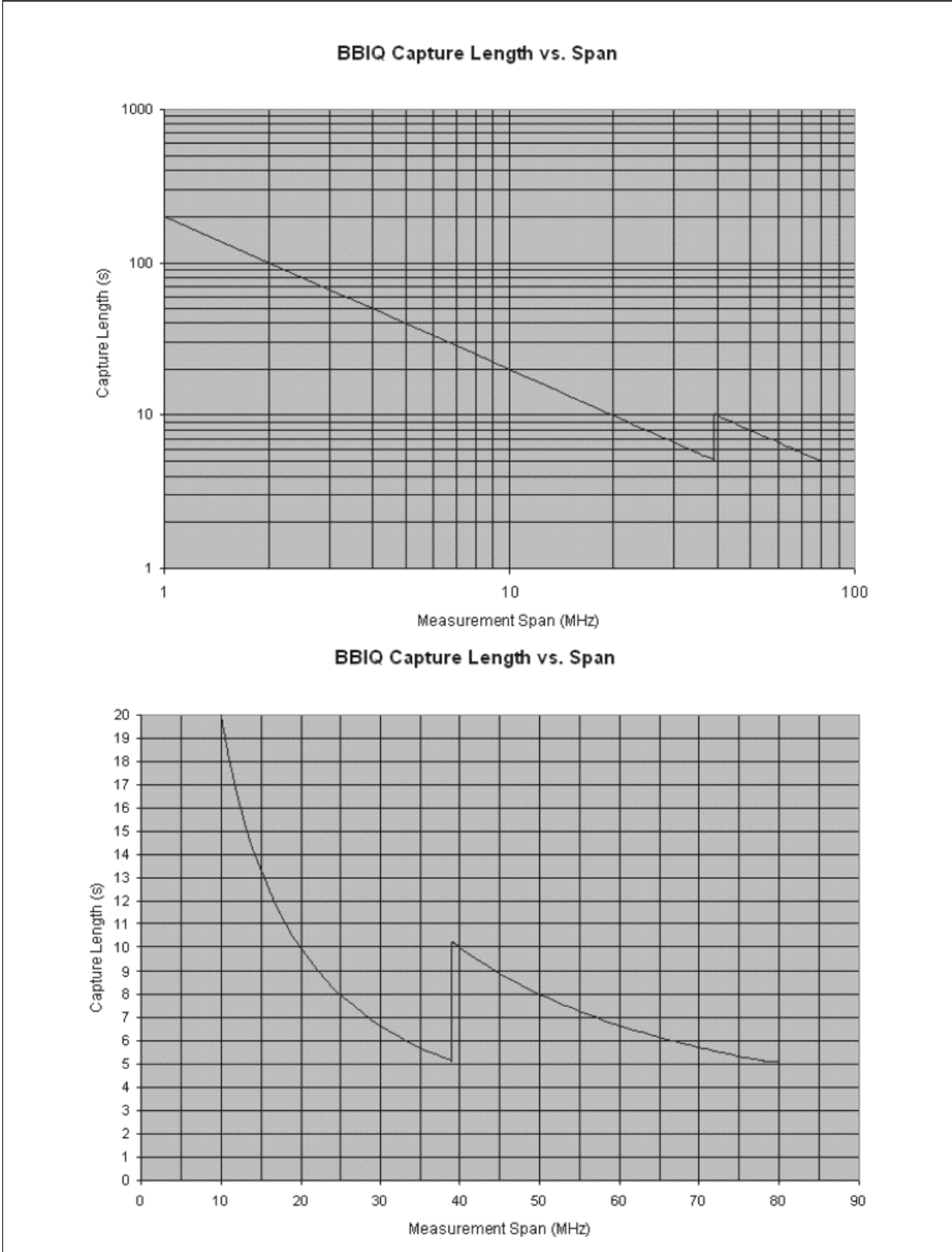
Capture Length vs. Span, 2-channel with 89600 VSA, I+jQ Mode [Plot]
